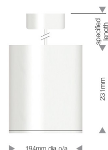
Suspension Dimensions
