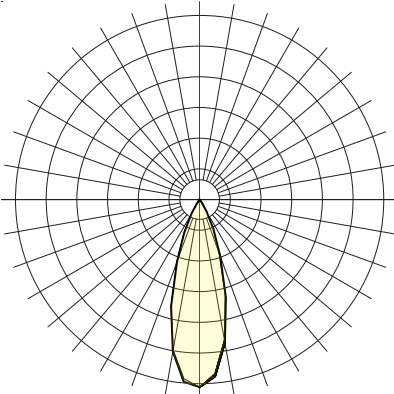
Nominal polar curve 15W, 35°, 4000K
